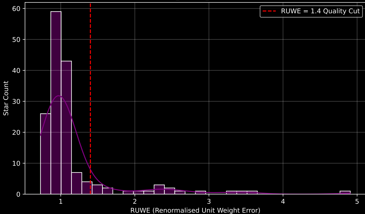
GAPOGEE DR17 Field [CVZTILE_103+22_btx] RUWE Distribution (n= 158)
